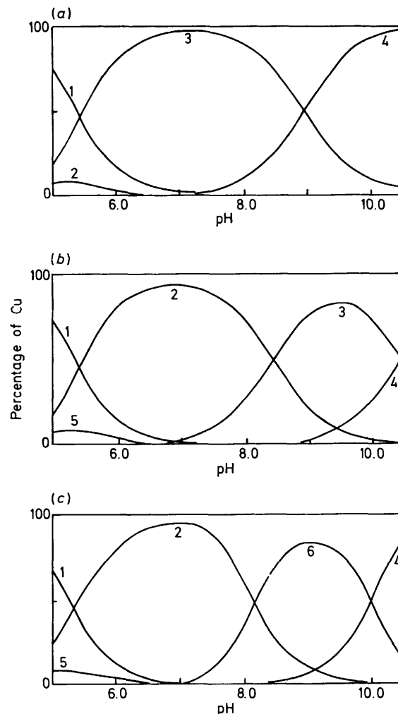
Figure 1. Species-distribution curves for 1:1 complexes of Cu 2+ with (a) Phe-Gly-Pro-Phe, (b) Phe-Gly-Pro-Tyr, and (c) Tyr-Gly-Pro-Phe (0.001 mol dm -3 ). Species. 1 = Cu 2+ , 2 = [CuL], 3 = [CuH 1 L], 4 = [CuH 2 L], 5 = [CuHL], and 6 = [CuH 1 L] 2 .
